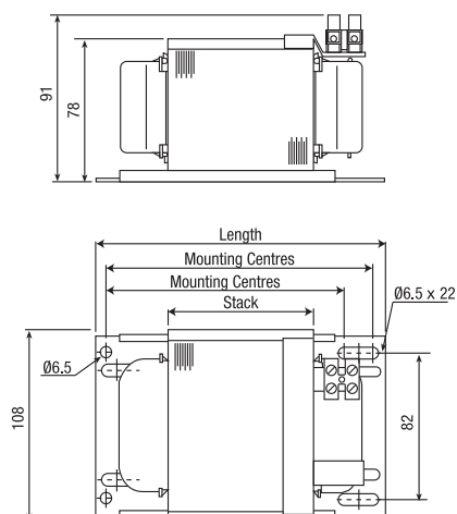
OG type ballasts with stack sizes 30–160 mm
