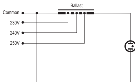
Leakage reactor ballast circuit for LPS lamps
