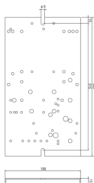
Gear tray for other applications
