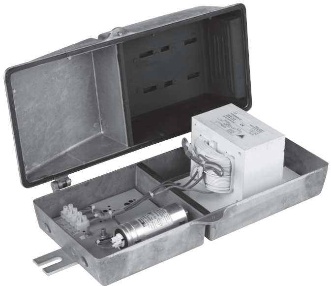
D96 weatherproof (IP65) enclosure
