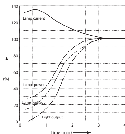
Similar to the mercury vapour lamps, metal halide lamps also require several minutes to develop full light output as is illustrated by the starting curves for a 400 W metal halide lamp
