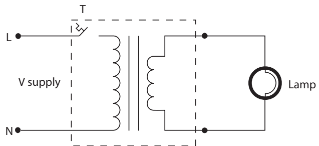
Low voltage lighting transformer circuit
