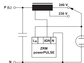
Multi-voltage circuit with pulse ignitors ZRM 4000 powerPULSE for sodium vapour lamps and metal halide lamps
