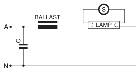
Switch start circuit
