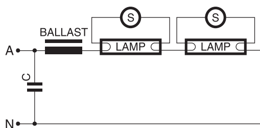
Twin series circuit
