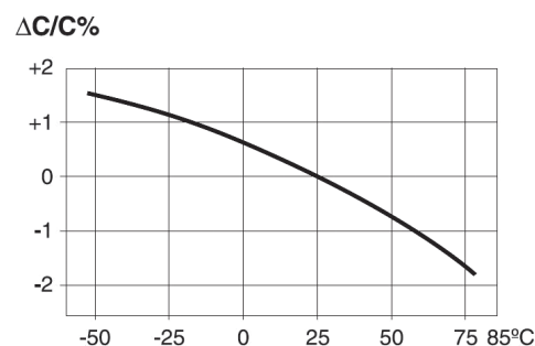
Capacitance versus Temperature
