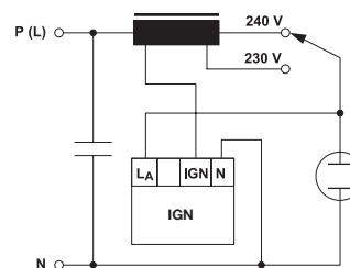
Multi-voltage circuit with pulse ignitors for sodium vapour lamps and metal halide lamps
