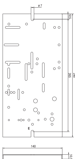
Gear tray to fit D430 box
